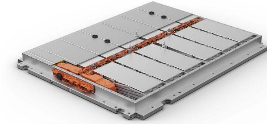
Example of a high-voltage battery from ID.4
